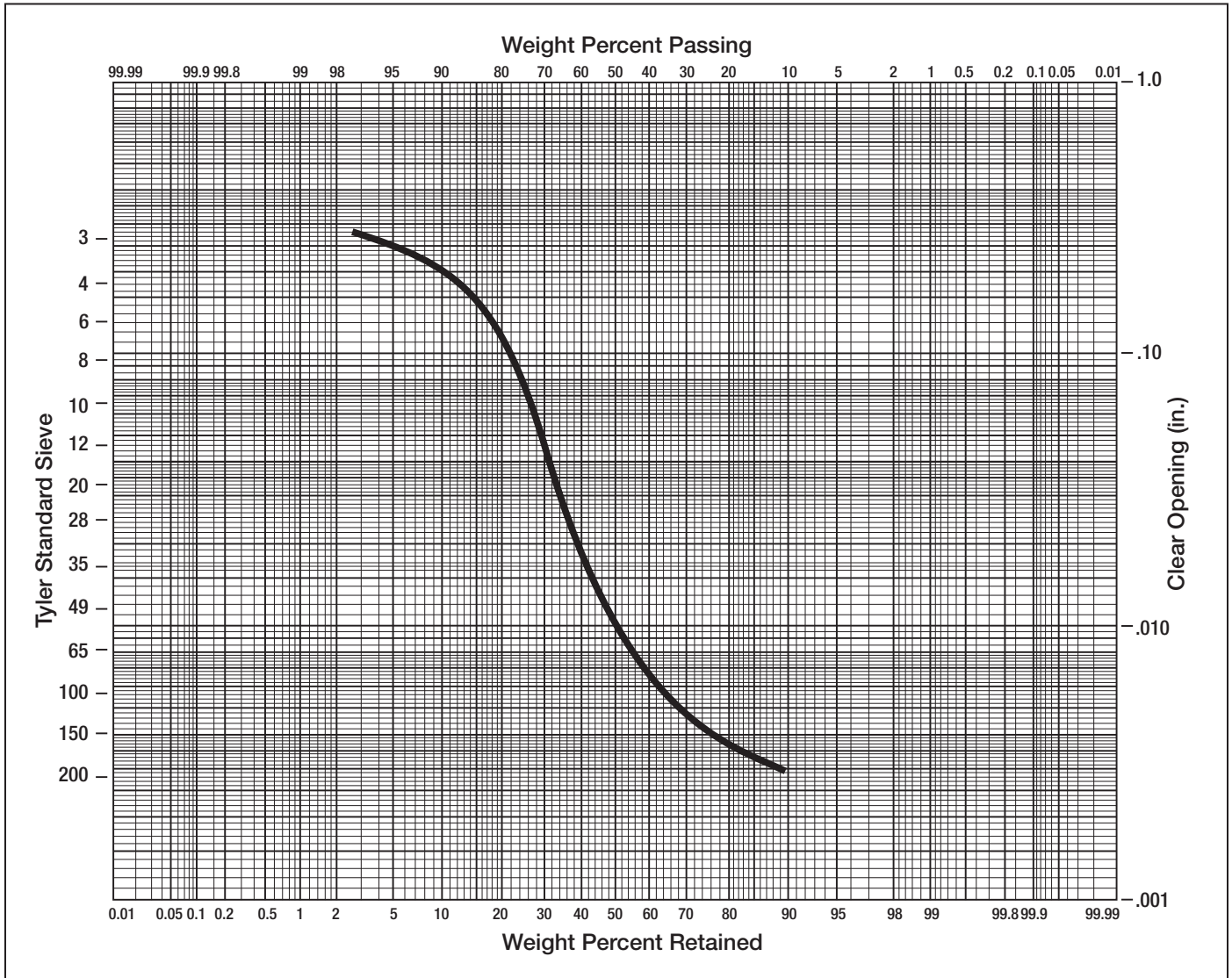
Figure 2: Communited limestone size distribution
